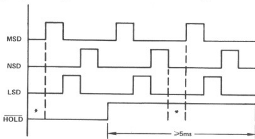
Figure 2. Timing Diagram
