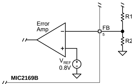
Figure 2. Voltage-Divider Configuration
