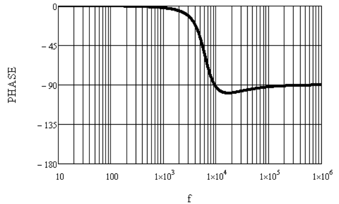
Figure 5. Phase Curve for G(s)
