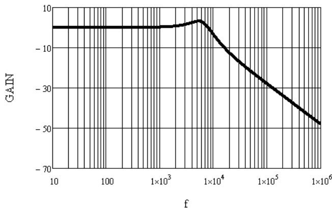
Figure 4. The Gain Curve for G(s)
