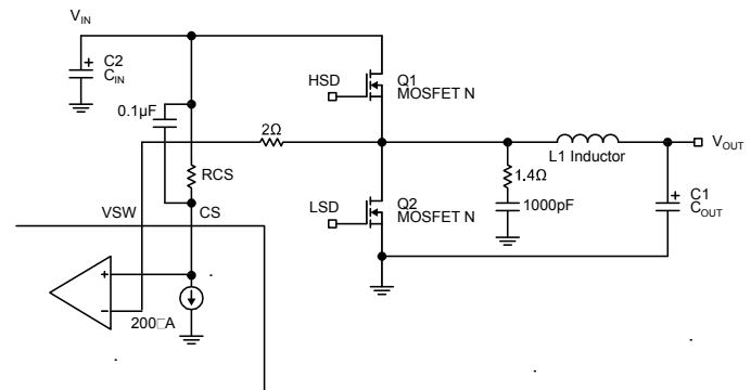
Figure 1. The MIC2169B Current Limiting Circuit
