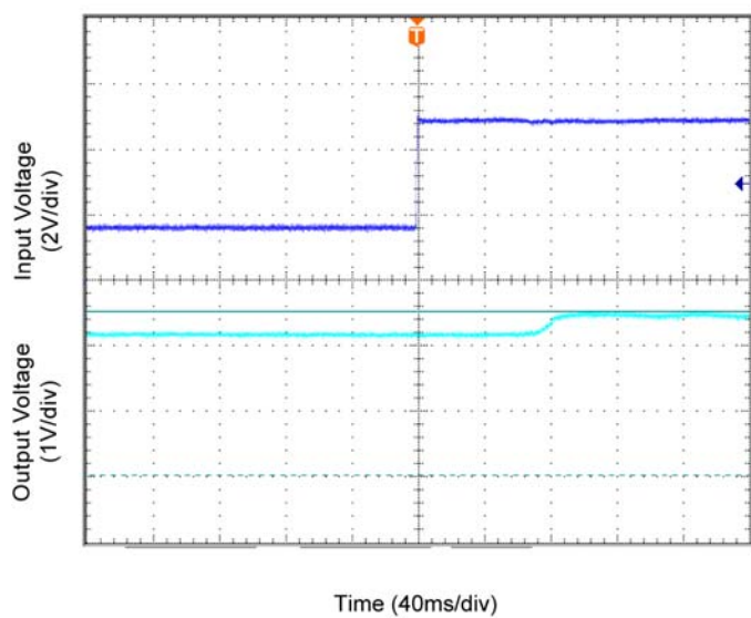
Fig 13 MIC2169B startup with pre-bias support, pre-bias at 90% of V_{out\_final}
