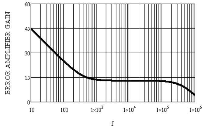
Figure 7. Error Amplifier Gain Curve
