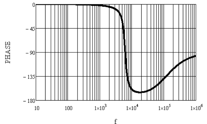
Figure 6. The Phase Curve with ESR = 0.002Ω
