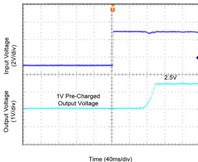
Figure 12. MIC2169B startup with pre-bias support
