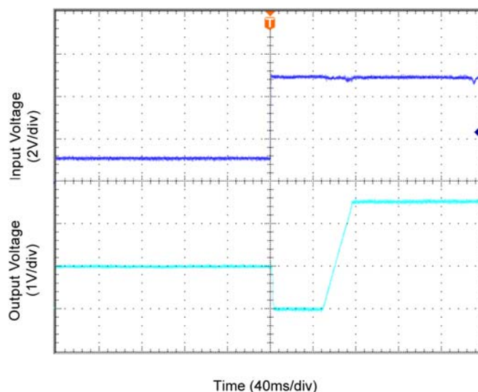
Figure 11. MIC2169A Startup without Pre-Bias Support
