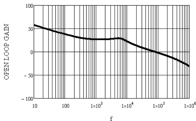
Figure 9. Open-Loop Gain Margin
