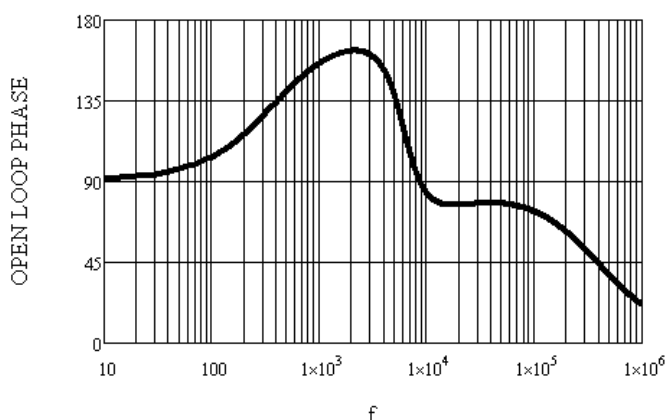
Figure 10. Open-Loop Phase Margin
