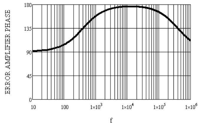
Figure 8. Error Amplifier Phase Curve
