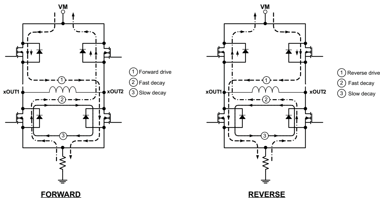
Figure 2. Current Paths
