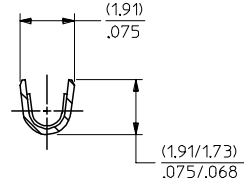
SECT. "B-B" SCALE:10X
