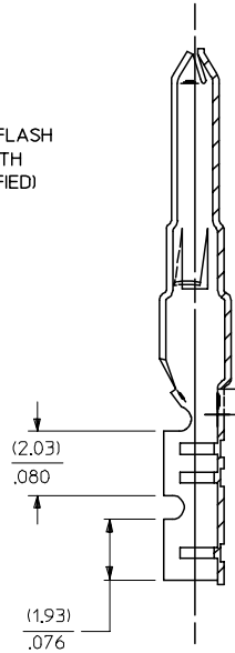
SECT. "A-A"
