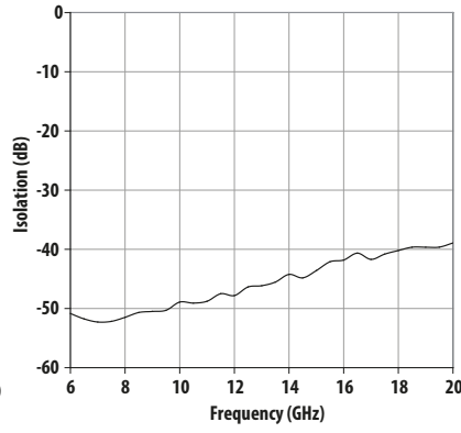
Figure 2. Typical Isolation
