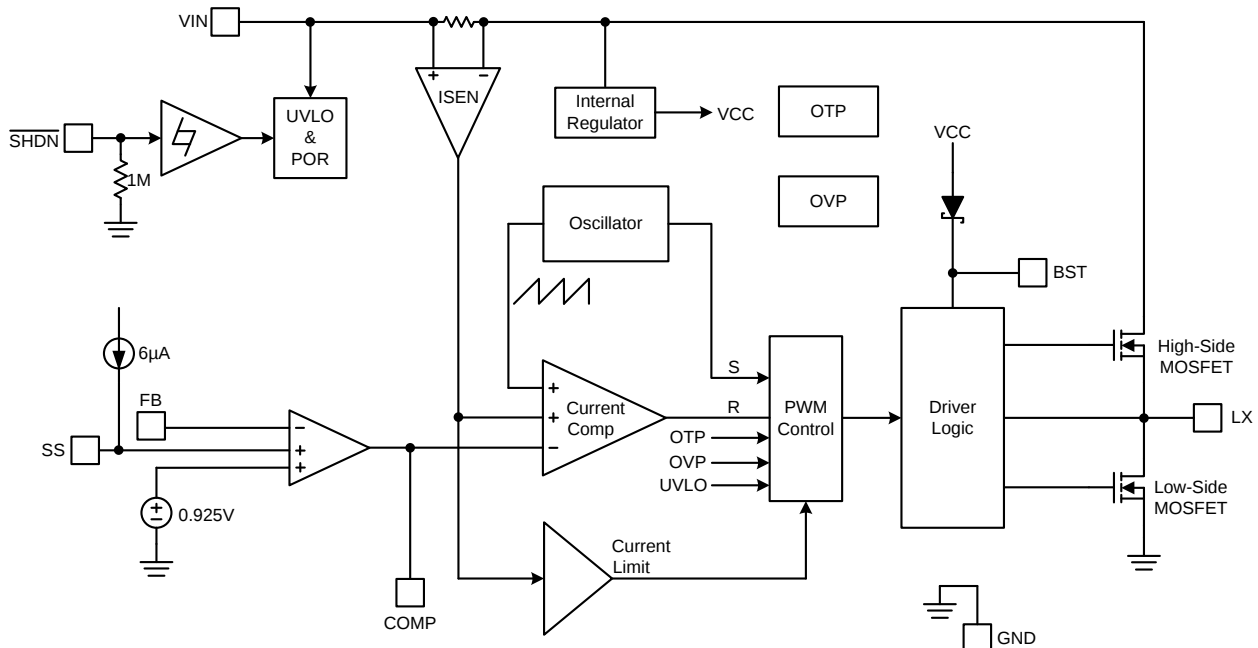
Figure 4. Block Diagram of FR9886C
