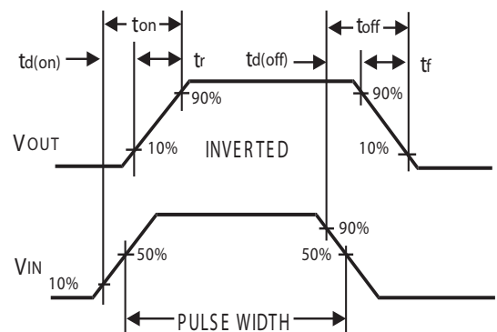
FIG.12 Switching Waveforms
