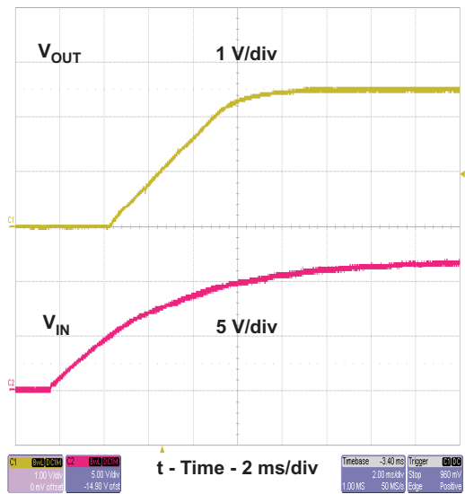
Figure 22. TPS54332 Start Up
