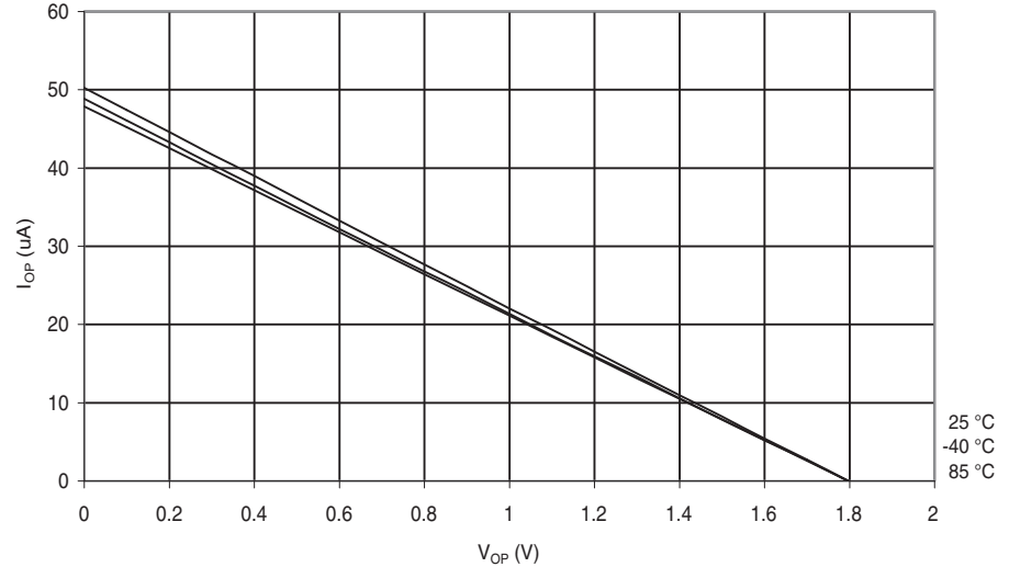
Figure 30-61. I/O Pin Pull-up Resistor Current vs. Input Voltage ( V_{CC} = 1.8 V).
