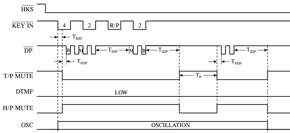
Figure 4. Pause Function
