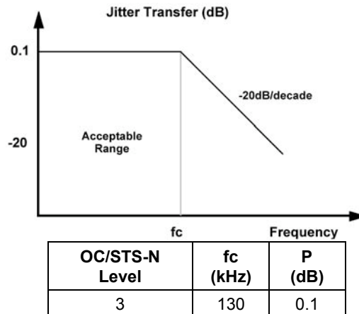
Figure 2. Jitter Transfer
