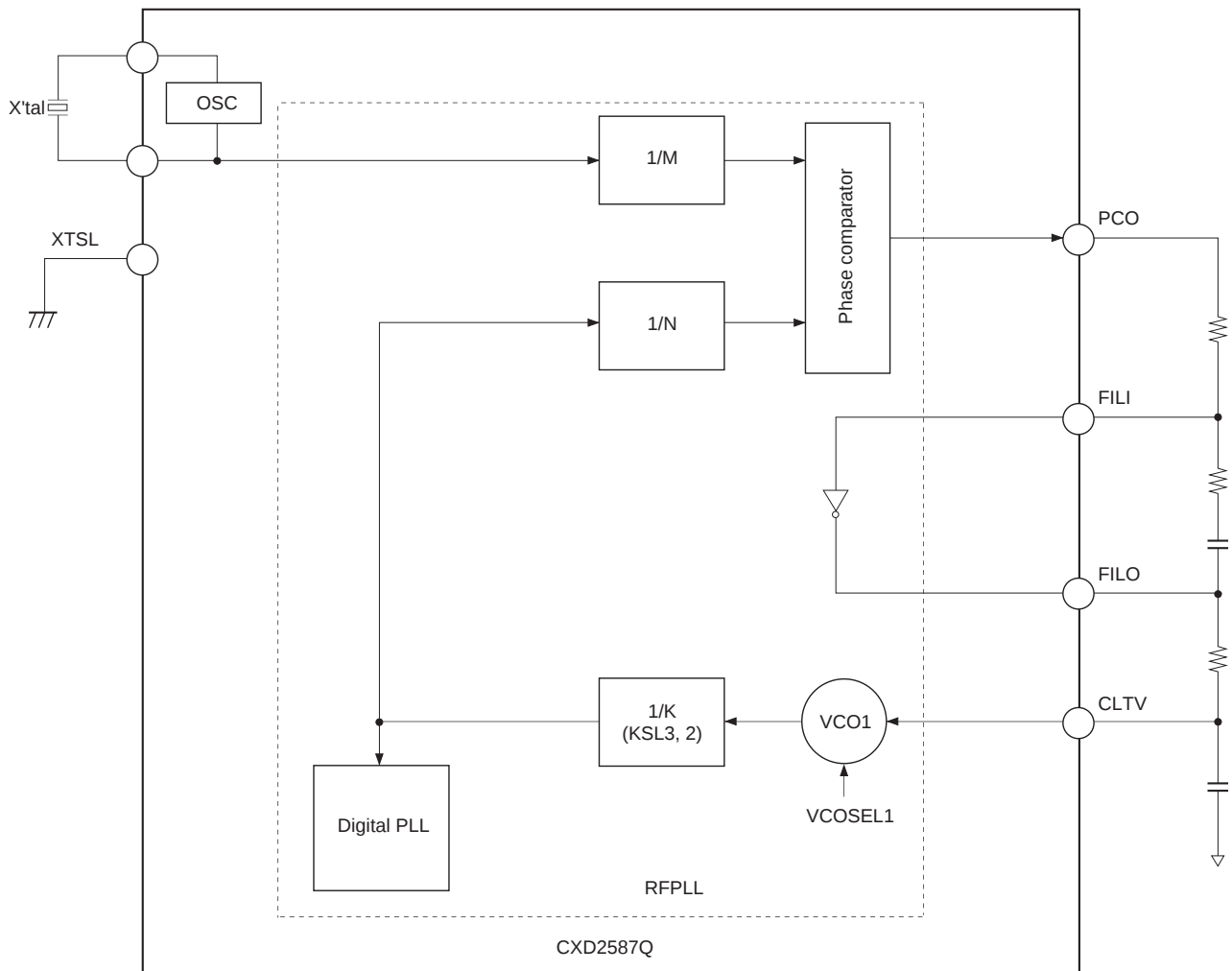
Block Diagram 3-1
