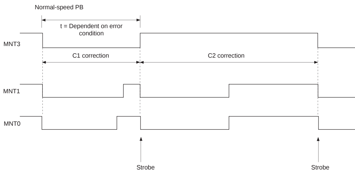
Timing Chart 3-3
