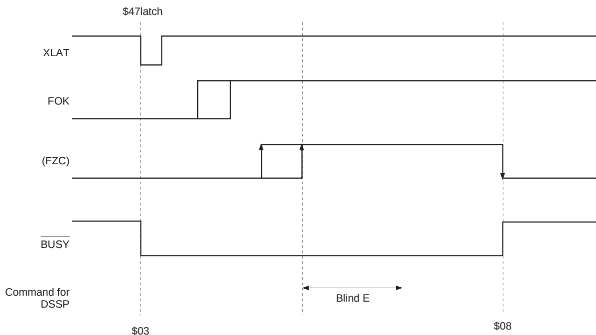
Fig. 3-6-(b). Auto Focus Timing Chart
