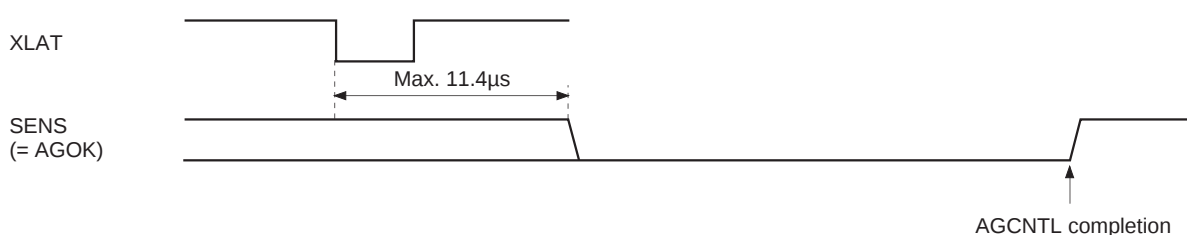
Timing Chart 4-4.
