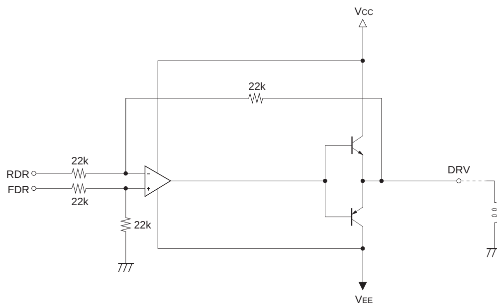
Fig. 4-21. Driver Circuit
