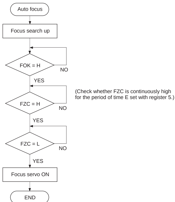
Fig. 3-6-(a). Auto Focus Flow Chart
