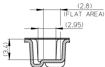
SECT Y-Y
