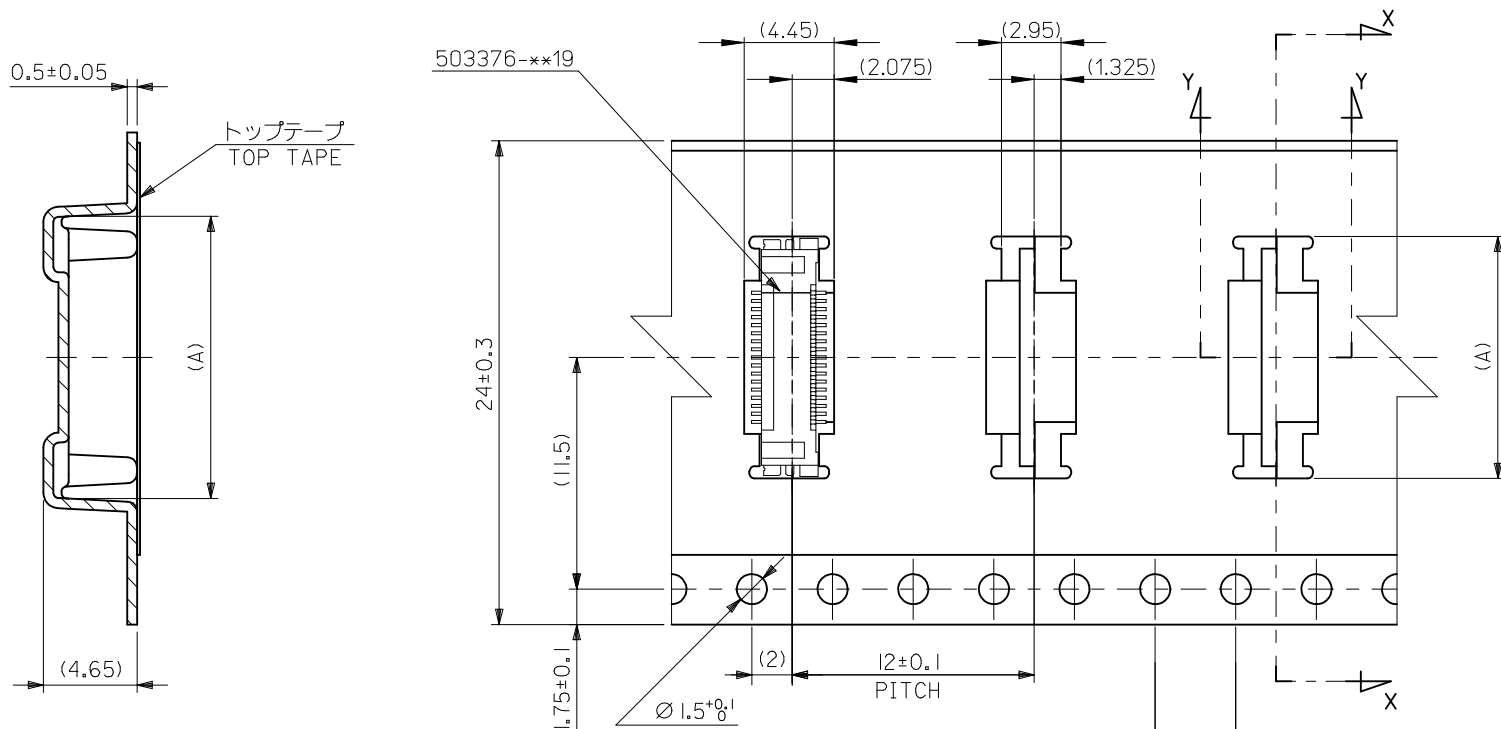
SECT X-X
