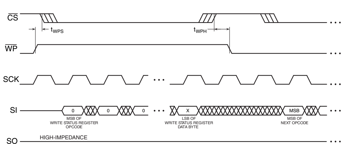
Figure 15-3. \overline{\text{WP}} Timing for Write Status Register Command When BPL = 1
