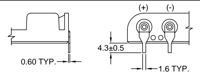
PDSN-18D PCB PINS
