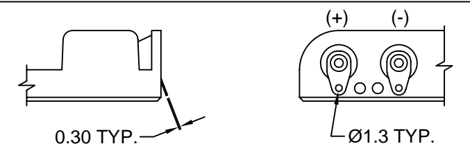
PDSN-18C SOLDER LUGS
