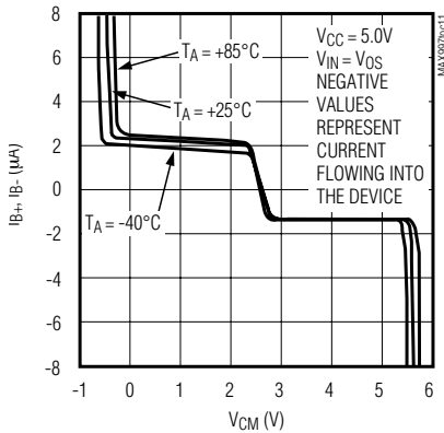
INPUT BIAS CURRENT ( I_{B+} , I_{B-} ) vs. COMMON-MODE VOLTAGE
