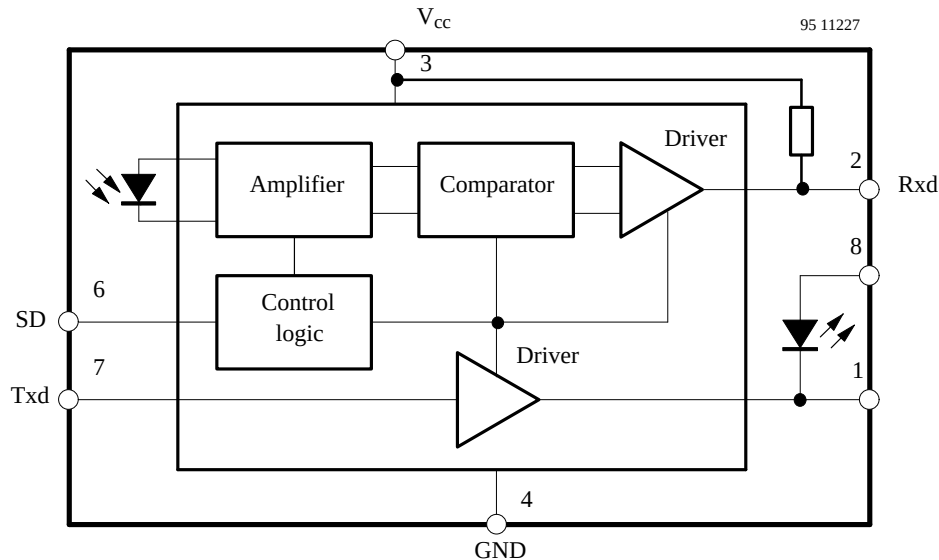
Figure 1. Block diagram
