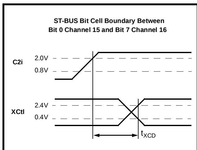
Figure 16 - XCtl Timing
