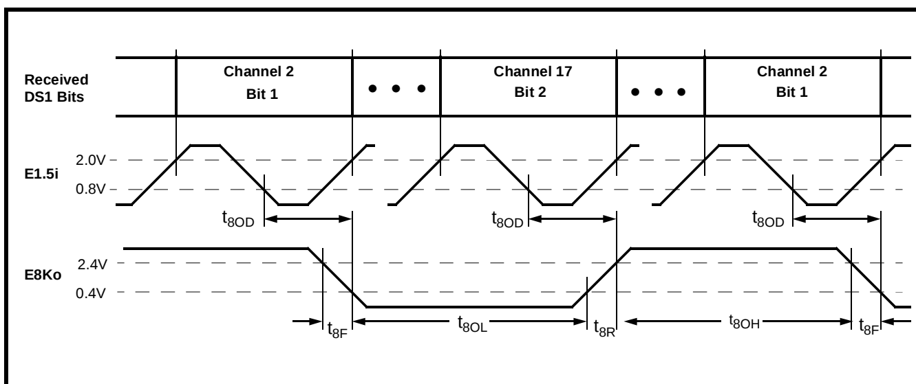
Figure 18 - E8Ko Timing
