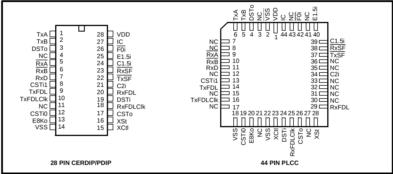
Figure 2 - Pin Connections
