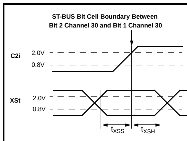
Figure 17 - XSt Timing
