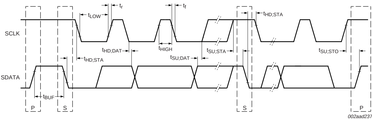
Fig 11. Timing measurements
