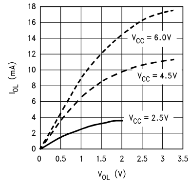
Port L/C/G Push-Pull Sink Current
