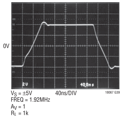
\pm 5V Large-Signal Response
