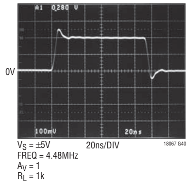
\pm 5V Small-Signal Response
