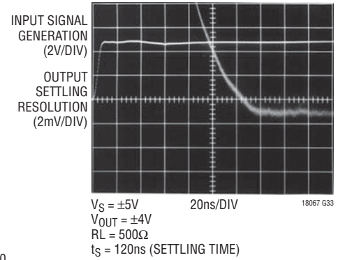
0.01% Settling Time
