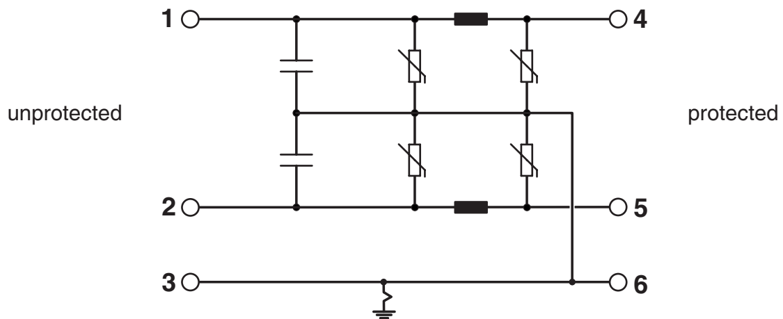
Circuit diagram
