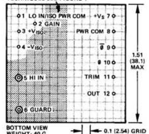
Model 286J
