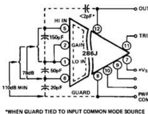
Figure 8. Model 286J Terminal Capacitance and CMR Ratings
