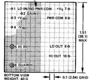
Model 284J
