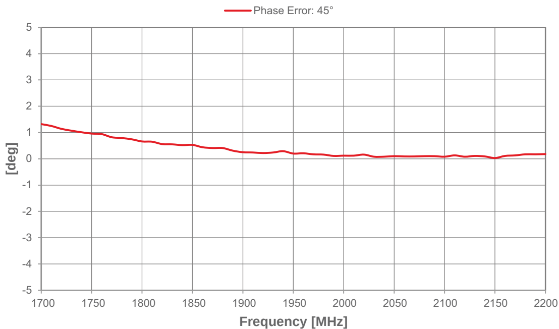
Figure 9 • Relative Phase Error: 22.5 Deg Bit
