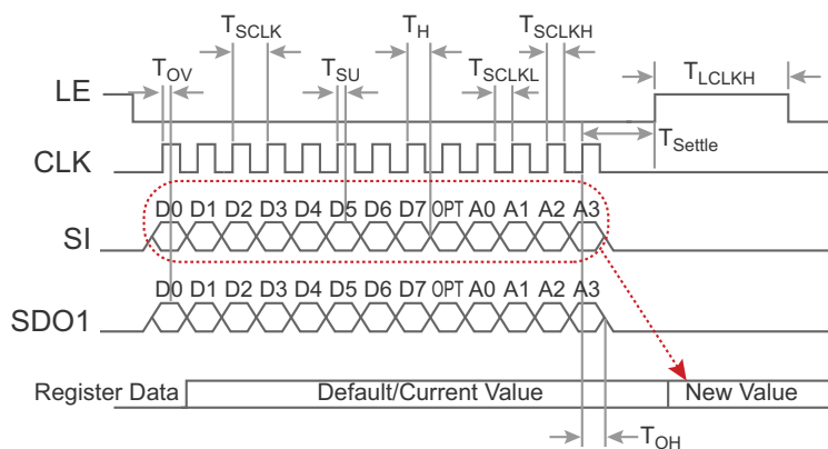
Figure 3 • Buffered SDO1 Serial Interface
