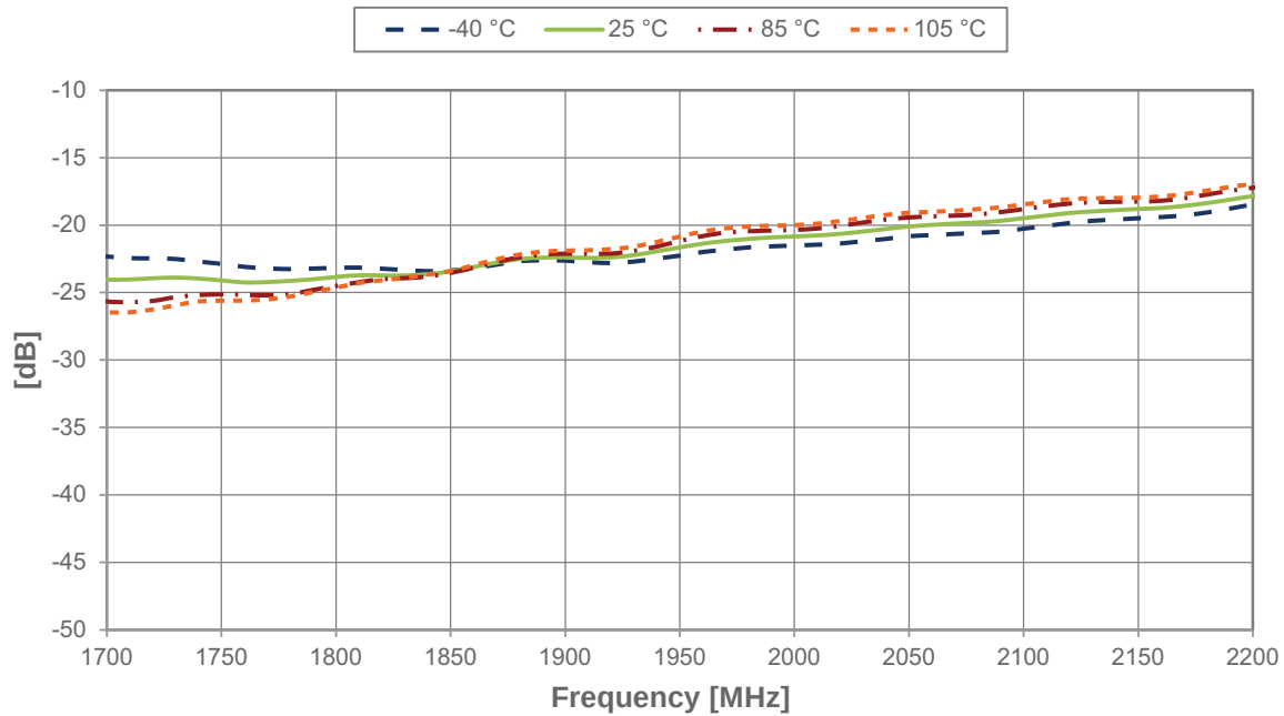
Figure 17 • Maximum Return Loss S_{22} Over All Major States
