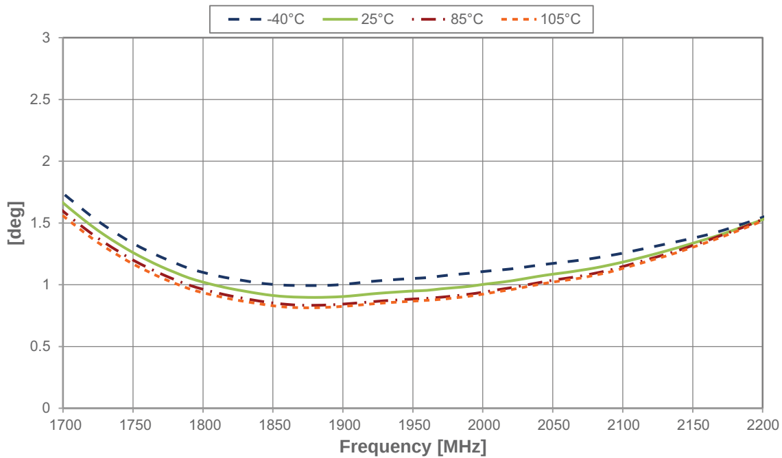
Figure 15 • RMS Phase Error
