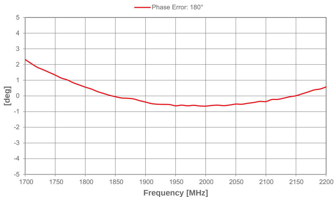
Figure 7 • Relative Phase Error: 90 Deg Bit
