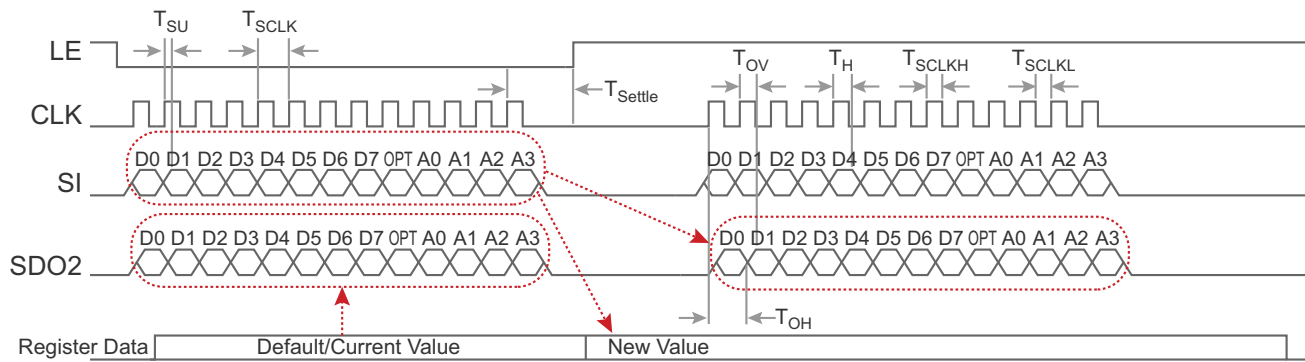
Figure 4 • SDO2 (Last Bit of Shift Register)—Single Write with Readback
