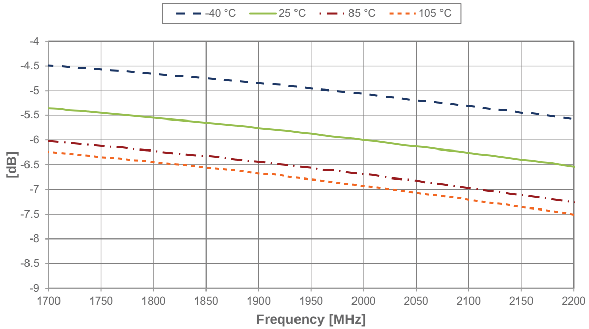
Figure 18 • Insertion Loss—Reference States
