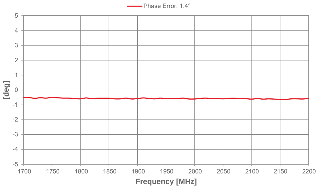
Figure 13 • Relative Phase Error: 1.4 Deg Bit
