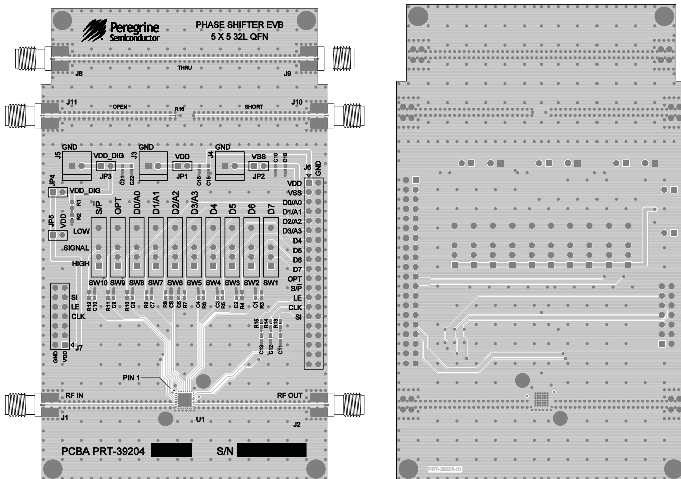
Figure 19 • Evaluation Kit Layout for PE44820
