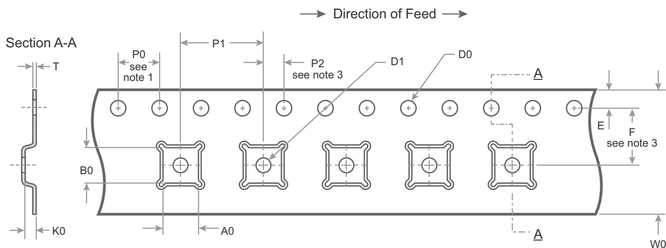
Figure 23 • Tape and Reel Specifications for 32-lead 5 \times 5 \times 0.85 mm QFN
