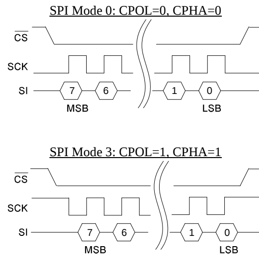
Figure 15. SPI Modes 0 & 3
