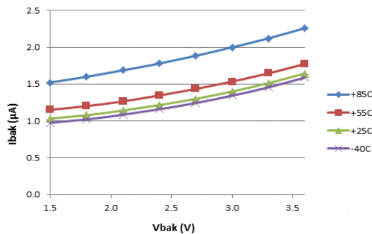
Figure 10. I_{BAK} vs. V_{BAK} Voltage
