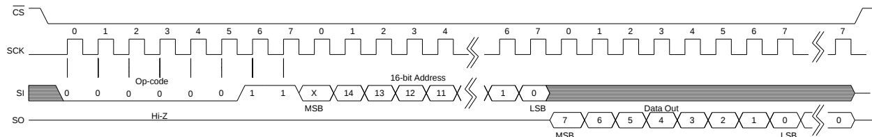
Figure 23. Memory Read
