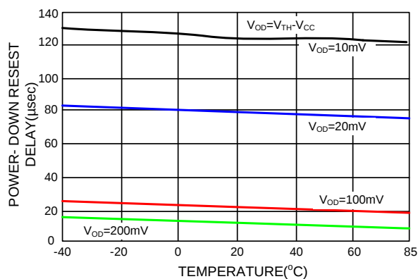
Figure 6. Power-Down Reset Delay vs Temperature and Overdrive(UM8xxL/M/J)
