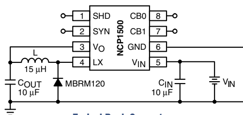
Typical Buck Converter
