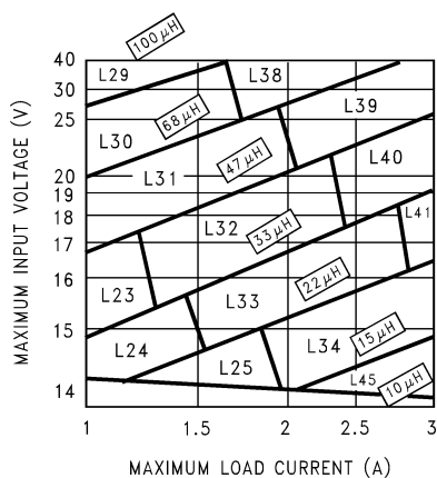
Figure 20. LM2673-12
