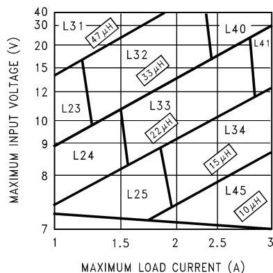
Figure 19. LM2673-5.0
