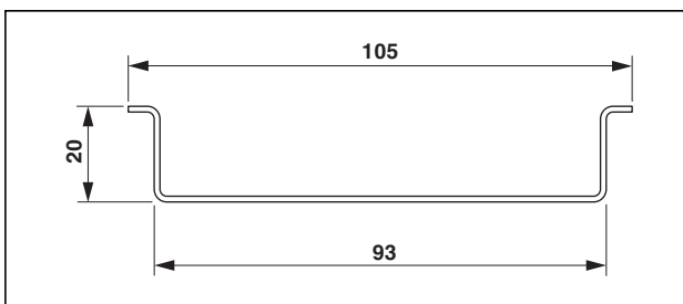
Figure 48 Dimensions NS 105/20
