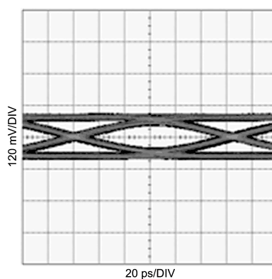
Figure 29. Equalized Signal (5m 26AWG Twin-AX Cable, 8Gbps, PRBS7)
