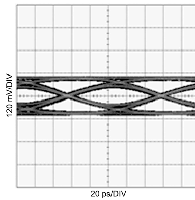
Figure 20. Equalized Signal (20in FR4, 10Gbps, PRBS7)
