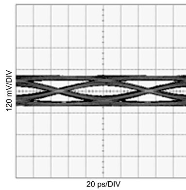
Figure 32. Equalized Signal (5m 26AWG Twin-AX Cable, 10Gbps, PRBS7)
