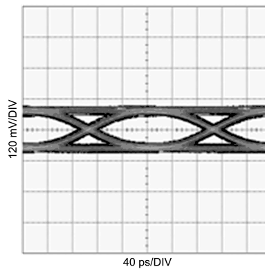
Figure 26. Equalized Signal (5m 26AWG Twin-AX Cable, 5Gbps, PRBS7)
