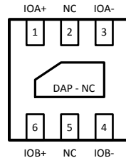
Figure 1. Bottom View 2.2mm x 2.5mm 6-Pin LLP Package Package Number SDA14A
