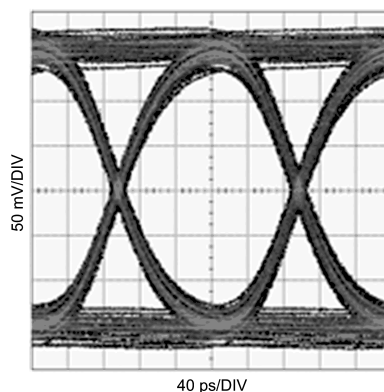
Figure 12. Equalized Signal (Zoom) (20in FR4, 5Gbps, PRBS7)
