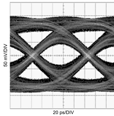
Figure 33. Equalized Signal (Zoom) (5m 26AWG Twin-AX Cable, 10Gbps, PRBS7)
