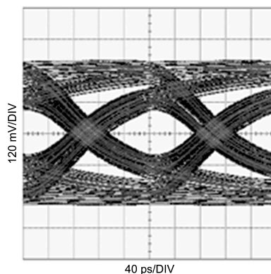
Figure 10. Unequalized Signal (20in FR4, 5Gbps, PRBS7)
