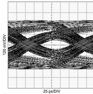
Figure 13. Unequalized Signal (20in FR4, 6.25Gbps, PRBS7)
