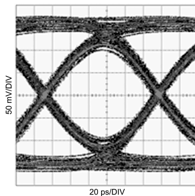
Figure 18. Equalized Signal (Zoom) (20in FR4, 8Gbps, PRBS7)
