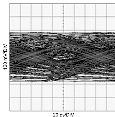
Figure 28. Unequalized Signal (5m 26AWG Twin-AX Cable, 8Gbps, PRBS7)
