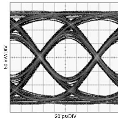
Figure 21. Equalized Signal (Zoom) (20in FR4, 10Gbps, PRBS7)
