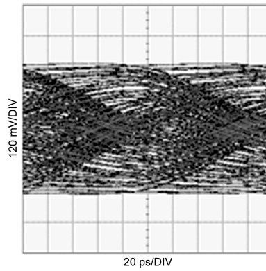
Figure 19. Unequalized Signal (20in FR4, 10Gbps, PRBS7)
