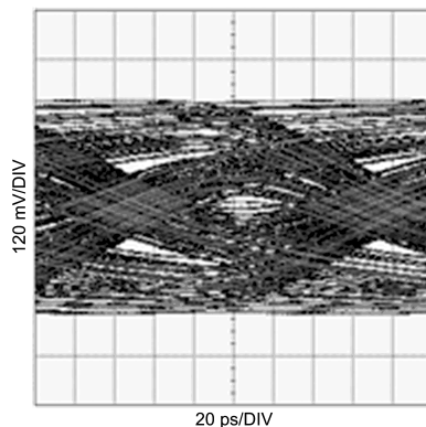
Figure 16. Unequalized Signal (20in FR4, 8Gbps, PRBS7)
