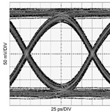
Figure 15. Equalized Signal (Zoom) (20in FR4, 6.26Gbps, PRBS7)
