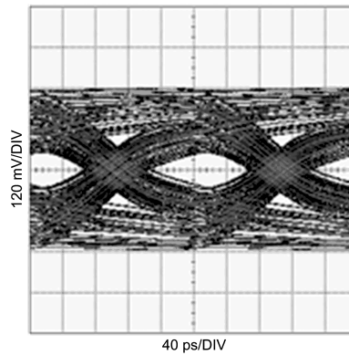
Figure 25. Unequalized Signal (5m 26AWG Twin-AX Cable, 5Gbps, PRBS7)
