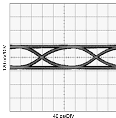
Figure 11. Equalized Signal (20in FR4, 5Gbps, PRBS7)
