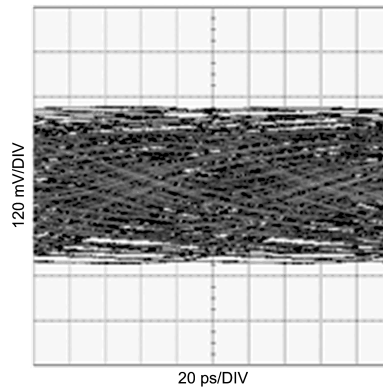
Figure 31. Unequalized Signal (5m 26AWG Twin-AX Cable, 10Gbps, PRBS7)
