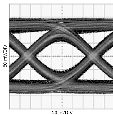
Figure 30. Equalized Signal (Zoom) (5m 26AWG Twin-AX Cable, 8Gbps, PRBS7)
