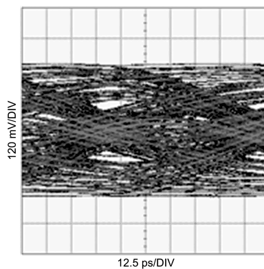
Figure 22. Unequalized Signal (14in FR4, 12.5Gbps, PRBS7)
