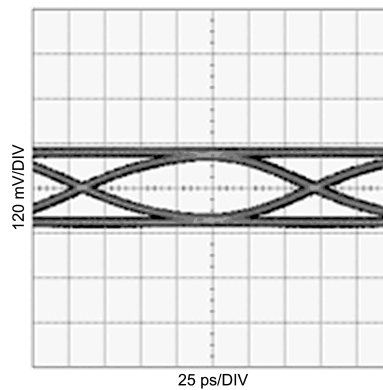
Figure 14. Equalized Signal (20in FR4, 6.25Gbps, PRBS7)
