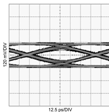
Figure 23. Equalized Signal (14in FR4, 12.5Gbps, PRBS7)
