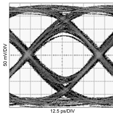
Figure 24. Equalized Signal (Zoom) (14in FR4, 12.5Gbps, PRBS7)
