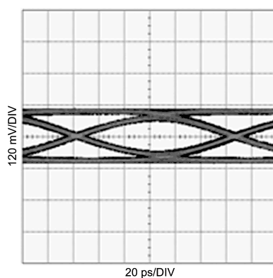
Figure 17. Equalized Signal (20in FR4, 8Gbps, PRBS7)
