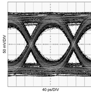
Figure 27. Equalized Signal (Zoom) (5m 26AWG Twin-AX Cable, 5Gbps, PRBS7)
