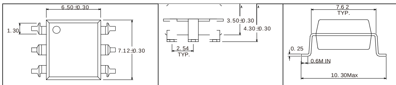
6-pin SOP
