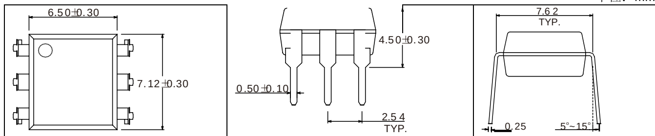
6-pin DIP
