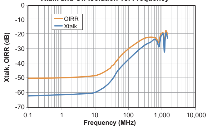
Xtalk and Off Isolation vs. Frequency
