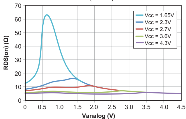
RDS(on) vs. Analog Voltage (at 25°C)
