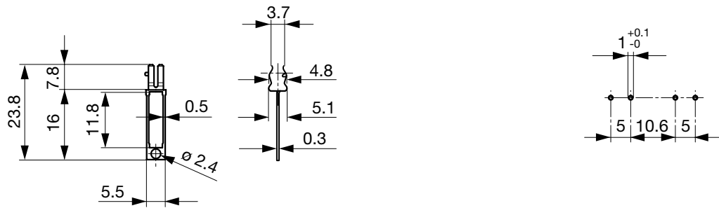
Drilling diagram
