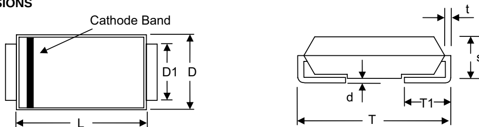
SMB/DO-214AA
