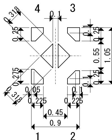
● USPQ-4B04 Reference Metal Mask Design
