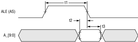
Figure 9. Microprocessor Interface Timing - Multiplexed Address
