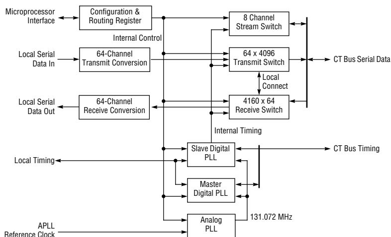
Figure 2. Block Diagram
