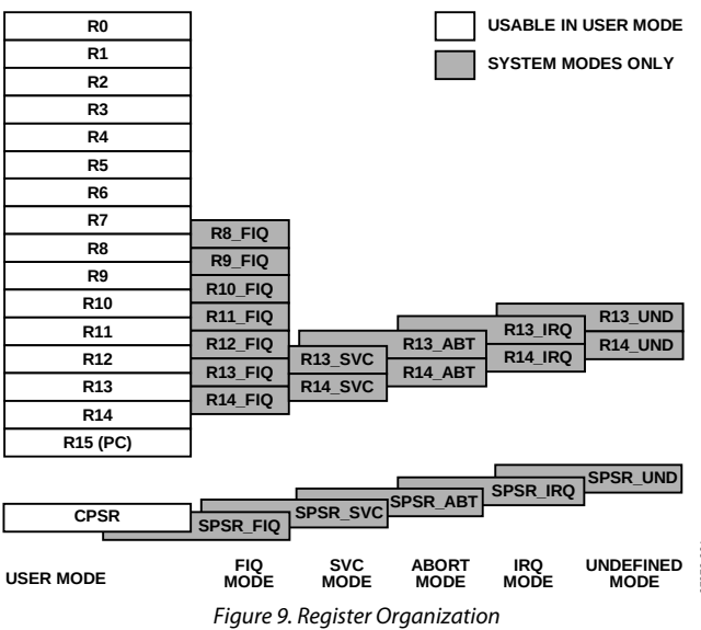
Figure 9. Register Organization
