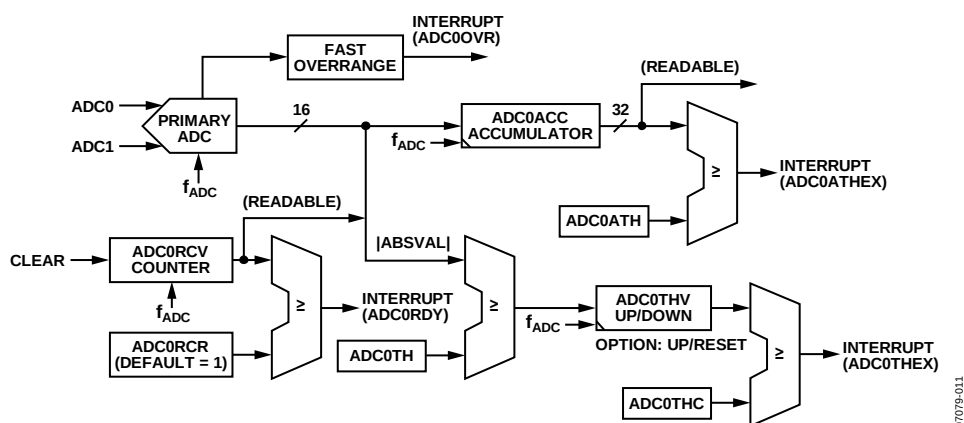
Figure 17. Primary ADC Accumulator/Comparator/Counter Block Diagram
