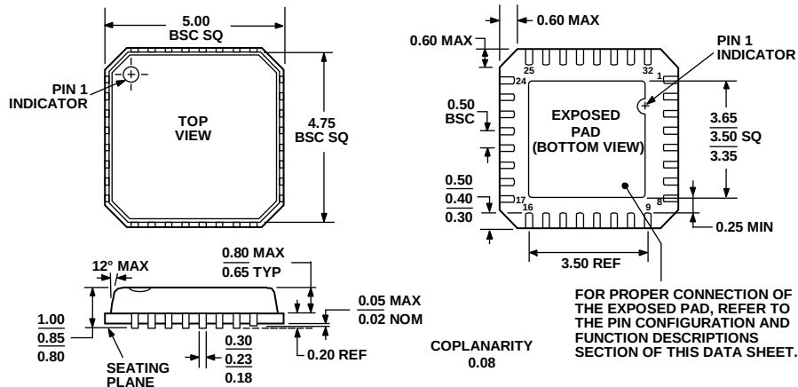
Figure 30. 32-Lead Lead Frame Chip Scale Package [LFCSP_VQ] 5 mm x 5 mm Body, Very Thin Quad (CP-32-4) Dimensions shown in millimeters
