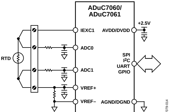
Figure 20. Example of an RTD Interface Circuit
