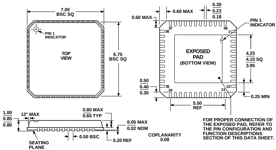
Figure 31. 48-Lead Lead Frame Chip Scale Package [LFCSP_VQ] 7 mm x 7 mm Body, Very Thin Quad (CP-48-3) Dimensions shown in millimeters
