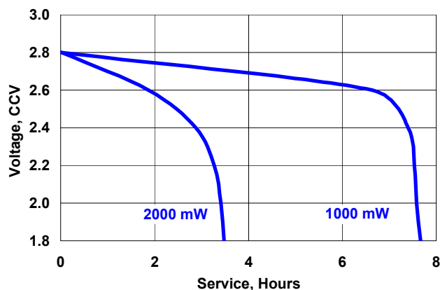
Typical Constant Power @21°C Continuous Discharge Characteristics
