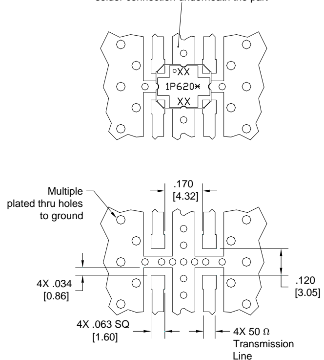
Dimensions are in Inches [Millimeters] 1P620* Rev A Mounting Footprint
