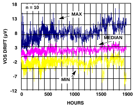
FIGURE 17. V_{OS} DRIFT SOIC vs TIME
