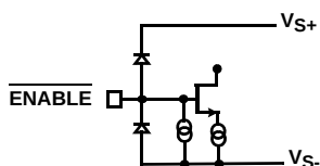
CIRCUIT 2
