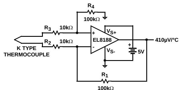
FIGURE 20. THERMOCOUPLE AMPLIFIER
