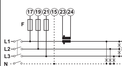
1-CT connection
