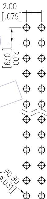
Recommended P.C.B Layout(Top Side) (PCB BOARD TOLERANCE±0.05)
