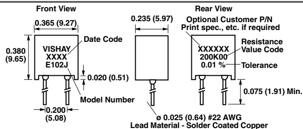
FIGURE 4 - STANDARD IMPRINTING AND DIMENSIONS
