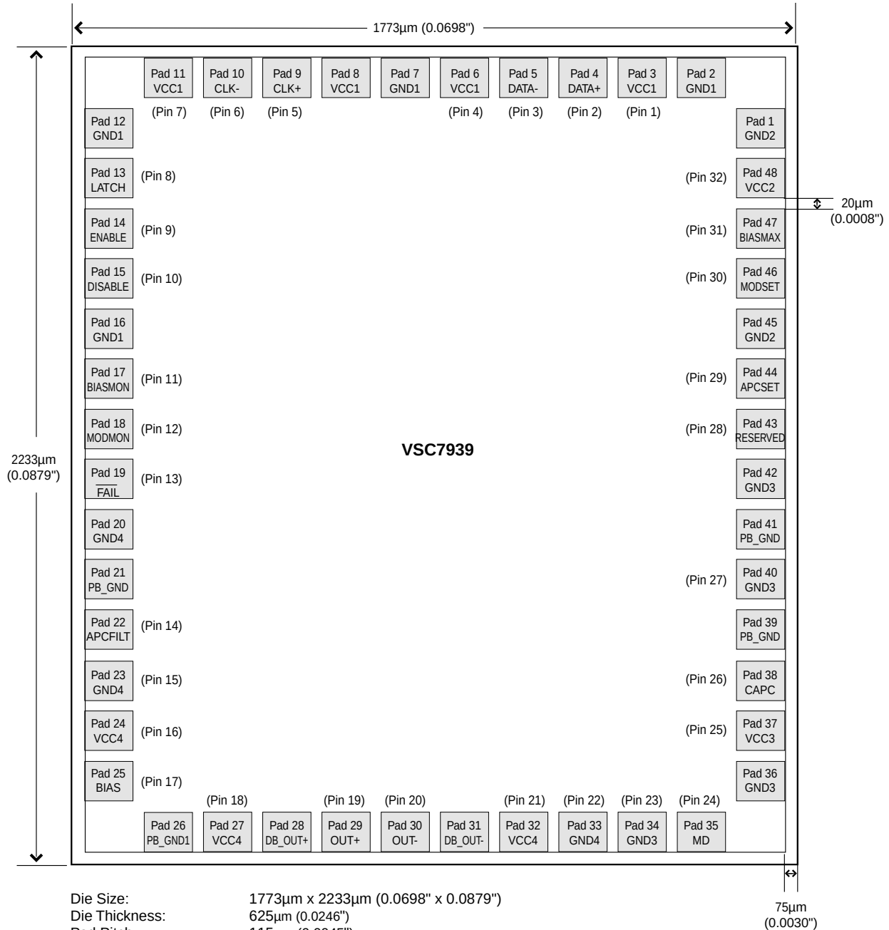
Figure 1: Pad Assignments
