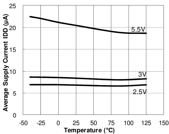
Average Supply Current vs. Temperature
