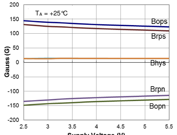
Switch Points vs Supply Voltage
