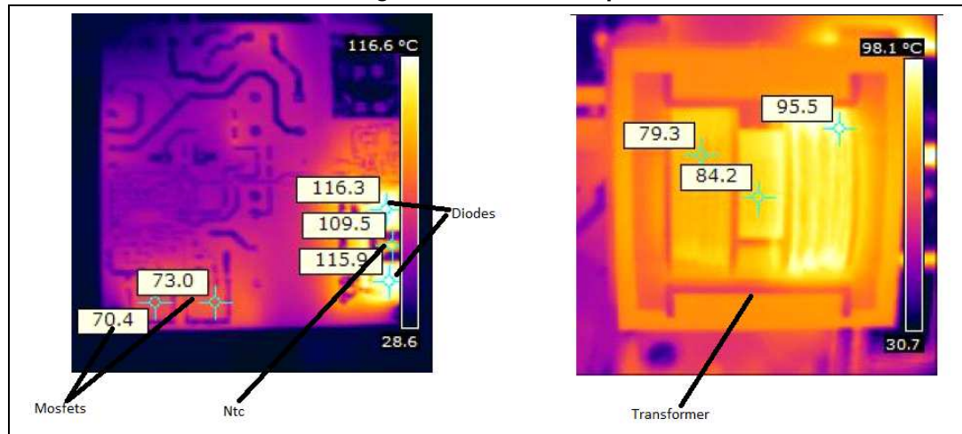
Figure 14. Thermal map
