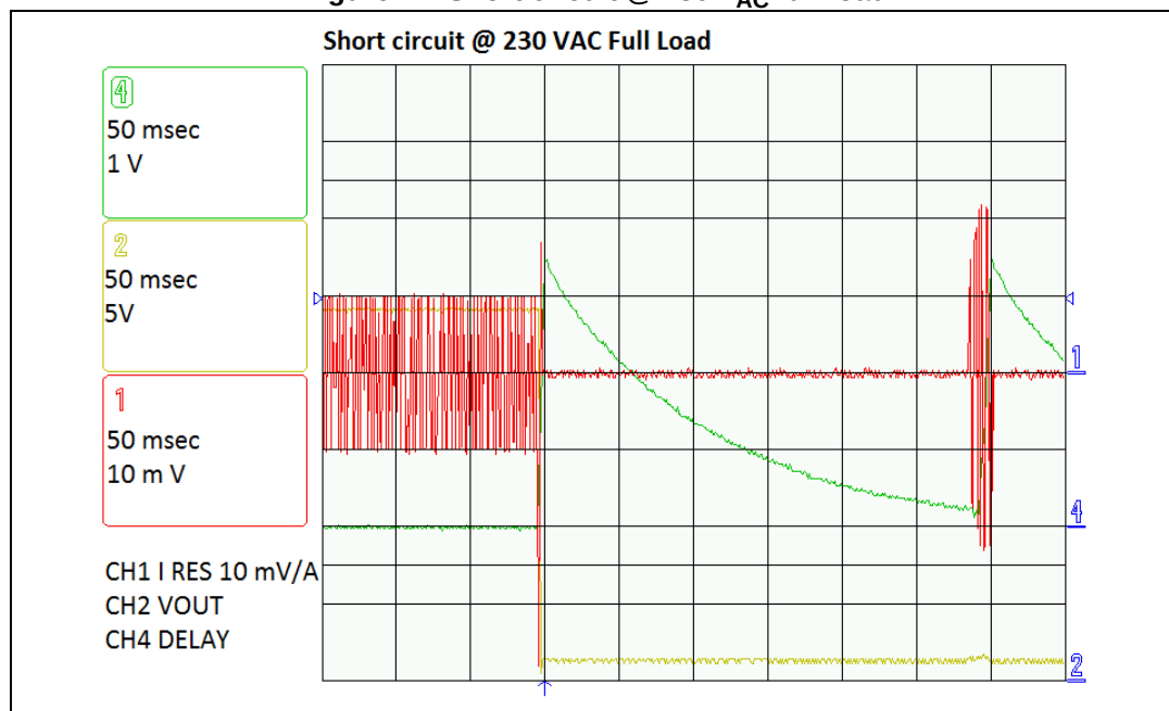
Figure 12. Short circuit @ 230 V AC full load
