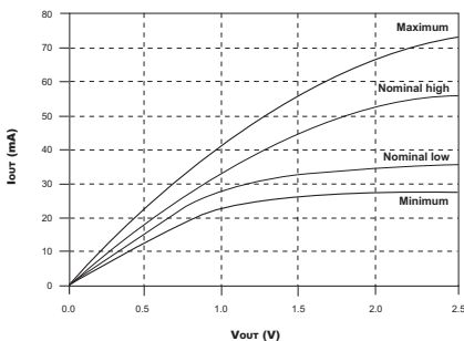
FIGURE C – PULL-DOWN CHARACTERISTICS
