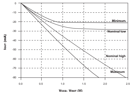
FIGURE D – PULL-UP CHARACTERISTICS
