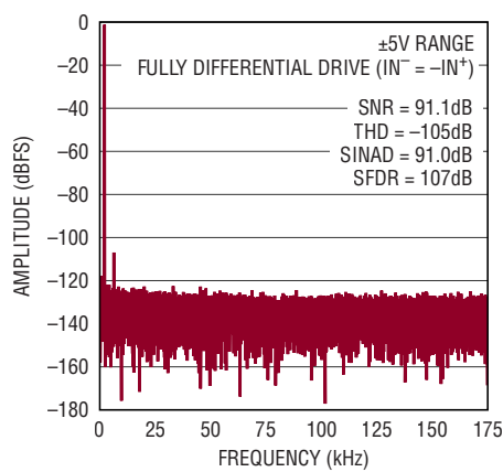
Figure 7c. IN + /IN - = 450mV 200Hz Fully Differential Sine, 0\text{V} \leq V_{CM} \leq 24\text{V} , 32k Point FFT, f_{SAMPL} = 350\text{kps} . Circuit Shown in Figure 7a
