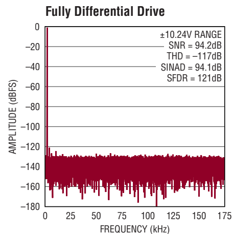
Figure 6c. IN^+/IN^- = -1\text{dBFS} 2kHz Fully Differential Sine, V_{\text{CM}} = 0\text{V} , 32k Point FFT, f_{\text{SAMPL}} = 350\text{ksps} . Circuit Shown in Figure 6a
