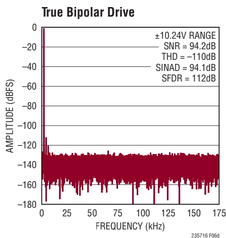
Figure 6d. IN^+ = -1\text{dBFS} 2kHz True Bipolar Sine, IN^- = 0\text{V} , 32k Point FFT, f_{\text{SAMPL}} = 350\text{ksps} . Circuit Shown in Figure 6a
