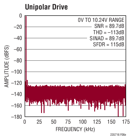
Figure 6e. IN^+ = -1\text{dBFS} 2kHz Unipolar Sine, IN^- = 0\text{V} , 32k Point FFT, f_{\text{SAMPL}} = 350\text{ksps} . Circuit Shown in Figure 6a
