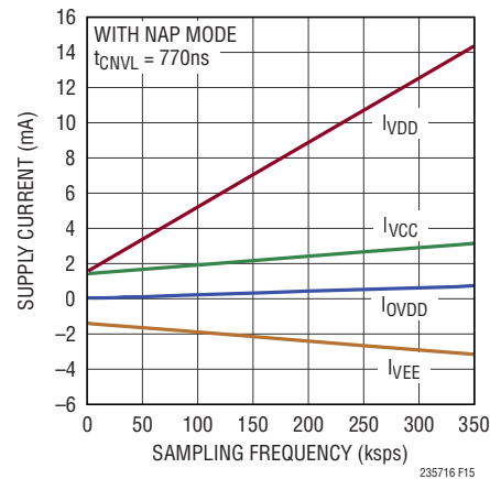
Figure 15. Power Dissipation of the LTC2357-16 Decreases with Decreasing Sampling Frequency
