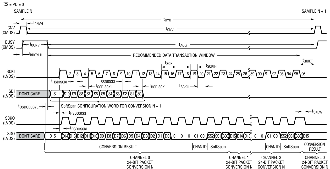
Figure 19. Serial LVDS I/O Mode
