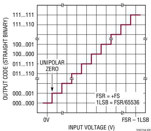
Figure 3. LTC2357-16 Straight Binary Transfer Function
