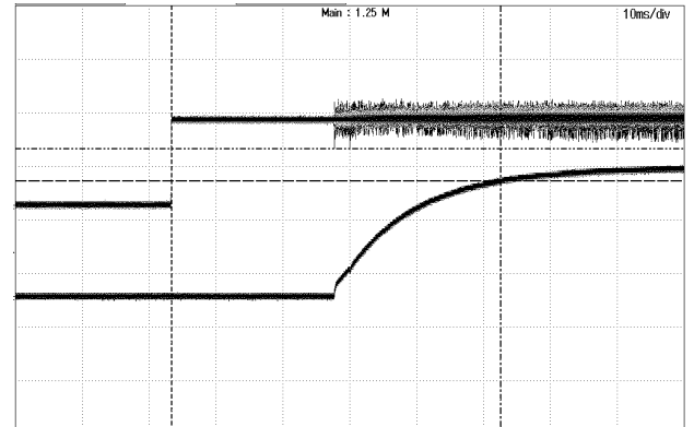
Figure 4: Turn-on transient at full load current (10ms/div). Top Trace: Vout; 5V/div; Bottom Trace: ON/OFF input: 2V/div.
