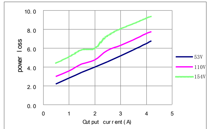
Figure 2: Power dissipation vs. load current for 53, 110 and 154V input voltage at 25°C.
