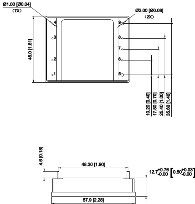
Figure 21 the pin function and mechanical drawing
