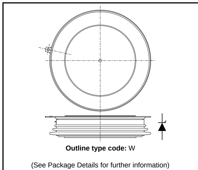
Fig. 1 Package outline
